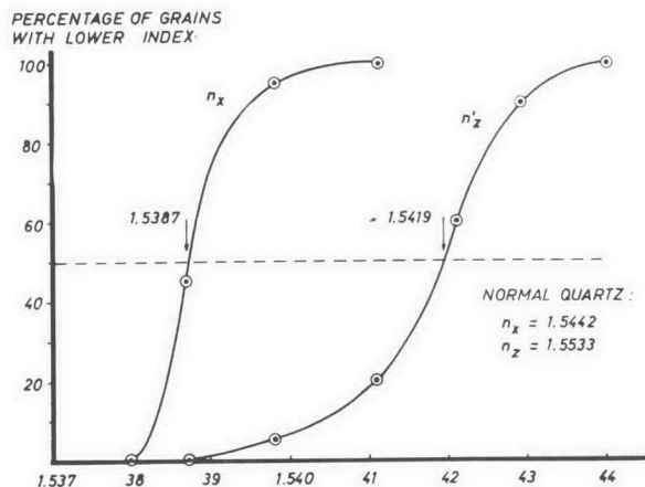
Fig. 5. Frequency distribution of refractive indices of quartz grains containing planar elements. Granite, West Clearwater Lake, Quebec.
